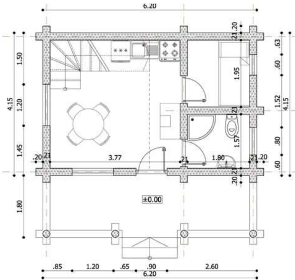
Plan parter S=25.73 mp
